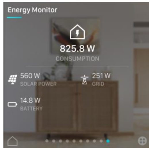
Figure 14 - Energy Monitor
